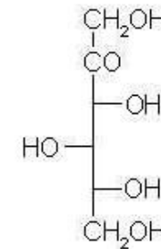
D-sorbosa
