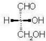
D-glyceraldehyd
