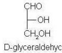
D-glyceraldehyd
