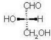
L-glyceraldehyd
