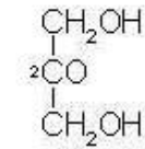
dihydroxyaceton
