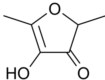
furaneol
