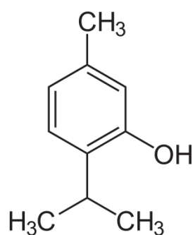
thymol
